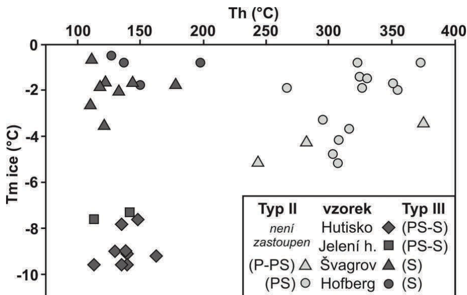
Obr. 1. Diagram Th vs. Tm ice pro FI s vodným roztokem typu II a III. Upraveno podle KROPÁČE et al. (2012). Fig. 1. Diagram Th vs. Tm ice for FI with the aqueous solution type II and III. Adjusted according to KROPÁČ et al. (2012).
